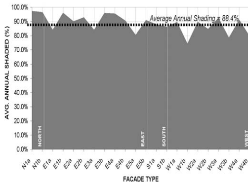
Fig 9. Overall average annual shading data (%)
