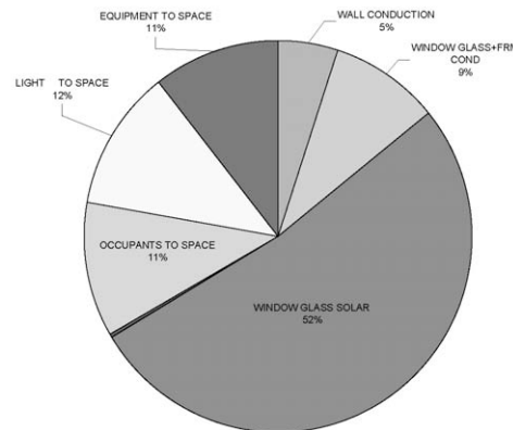
Fig 4. Typical office building cooling loads breakdown (Source; EDS, 2007)
