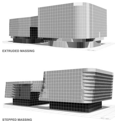
Fig 5. Insolation studies for extruded massing compared with stepped massing
