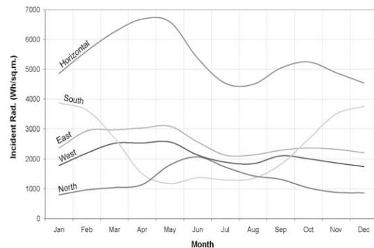
Fig 1. Incident Solar Radiation on Various Facades (Source; Meteonorm)
