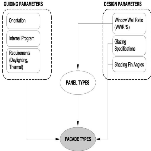
Fig 7. Façade design process
