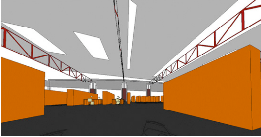
Fig 8. An early design alternative with diffuse skylights
