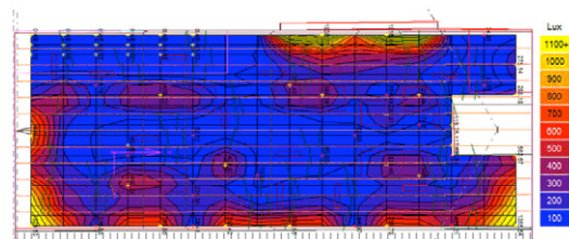
Fig 13. Illuminance values over the work plane for December 21 at noon under overcast sky conditions
